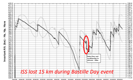
International Space Station As Flown Altitude Profile (Based on MCC-MUUSP Tracked SV Data)
