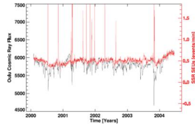
Figure 3: Subset of the data in Fig. 1 during solar maximum. The plot shows a dozen sharp spikes on top of the solar-cycles-modulated background of SSR SEUs triggered by cosmic ray hits. These spikes are caused by isolated strong SEP events. Most of them coincide with a CRF down spike.
