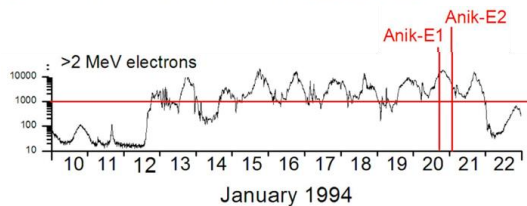
Fig. 7 from Lai et al. (2018): Deep Dielectric Charging and Spacecraft Anomalies
