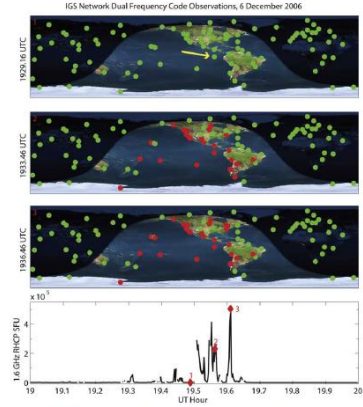
Figure 6. Receivers in the Global GPS Network that were analyzed during the solar radio burst. Green indicates the normal number of satellites being tracked. (4th panel) During the burst (power at 1.6 GHz), several sunlit receivers tracked fewer than the four satellites needed for a full positioning solution (marked in red). (Image of Earth from The Living Earth, 1996 and is used here by permission of the publisher. Day/night overlay created using Earth Viewer by J. Walker.)
