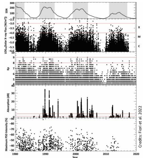
Figure from Fiori et al. 2022 - https://www.swsc-journal.org/articles/swsc/full_html/2022/01/swsc220003/swsc220003.html Occurrence rate and duration of space weather impacts on high-frequency radio communication used by aviation
