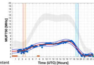
Credits: Peter Forister - https://www.facebook.com/PeterForisterPhoto Ionosphere Maximum Usable Frequency (MUF750) Date : 2023-03-24 Day Number : 083 Time : 23:33:16 [UTC]
