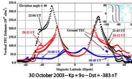
30 October 2003 – Kp = 9o – Dst = -383 nT
