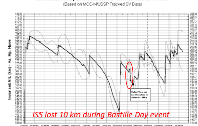
International Space Station As Flown Altitude Profile
