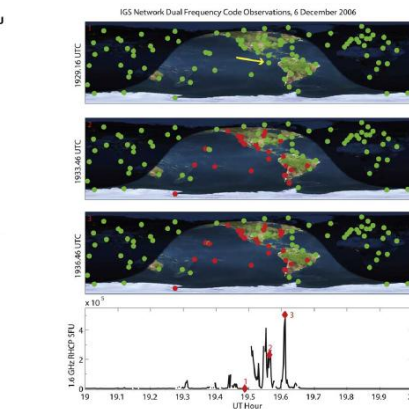
Figure 6. Receivers in the Global GPS Network that were analyzed during the solar radio burst. Green indicates the normal number of satellites being tracked. (fourth panel) During the burst (power at 1.6 GHz), several sunlit receivers tracked fewer than the four satellites needed for a full positioning solution (marked in red). (Image of Earth from the The Living Earth, 1996 and is used here by permission of the publisher. Day/night overlay created using Earth Viewer by J. Walker.)
