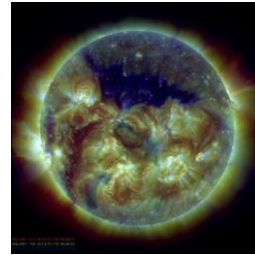
Coronal Holes
