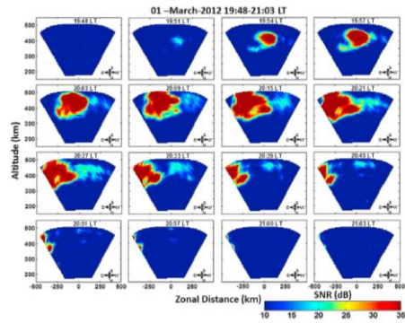
Figure 1. An example showing the genesis and successive development of EPB (Irregularity Free Region) over Kotabang observed from the fan sector maps of EAR on 1 March 2012.
