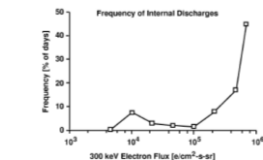
Figure 11. Comparison of SCATHA anomalies with energetic electron fluxes.
