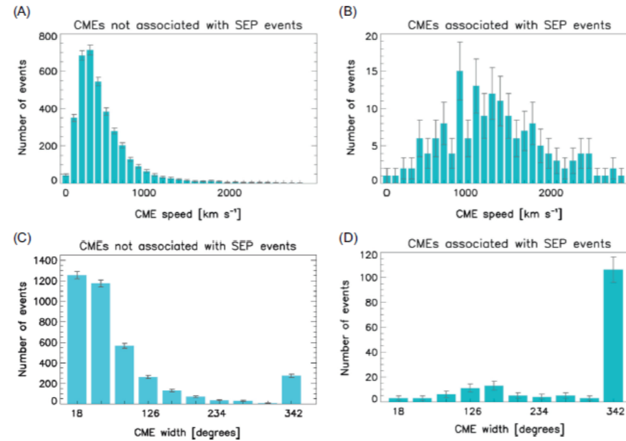
Fig. 6. Distribution of the CME velocity (in km s -1 ) for all 3535 CMEs not associated with SEP events in our sample from 1997–2013 (A) and for the 158 SEP events, within the same time period (B). Distribution of the CME width (in degrees) for all 3535 CMEs not associated with SEP events in our sample from 1997–2013 (C) and for the 158 SEP events, within the same time period (D). The error bars denote the statistical error.
