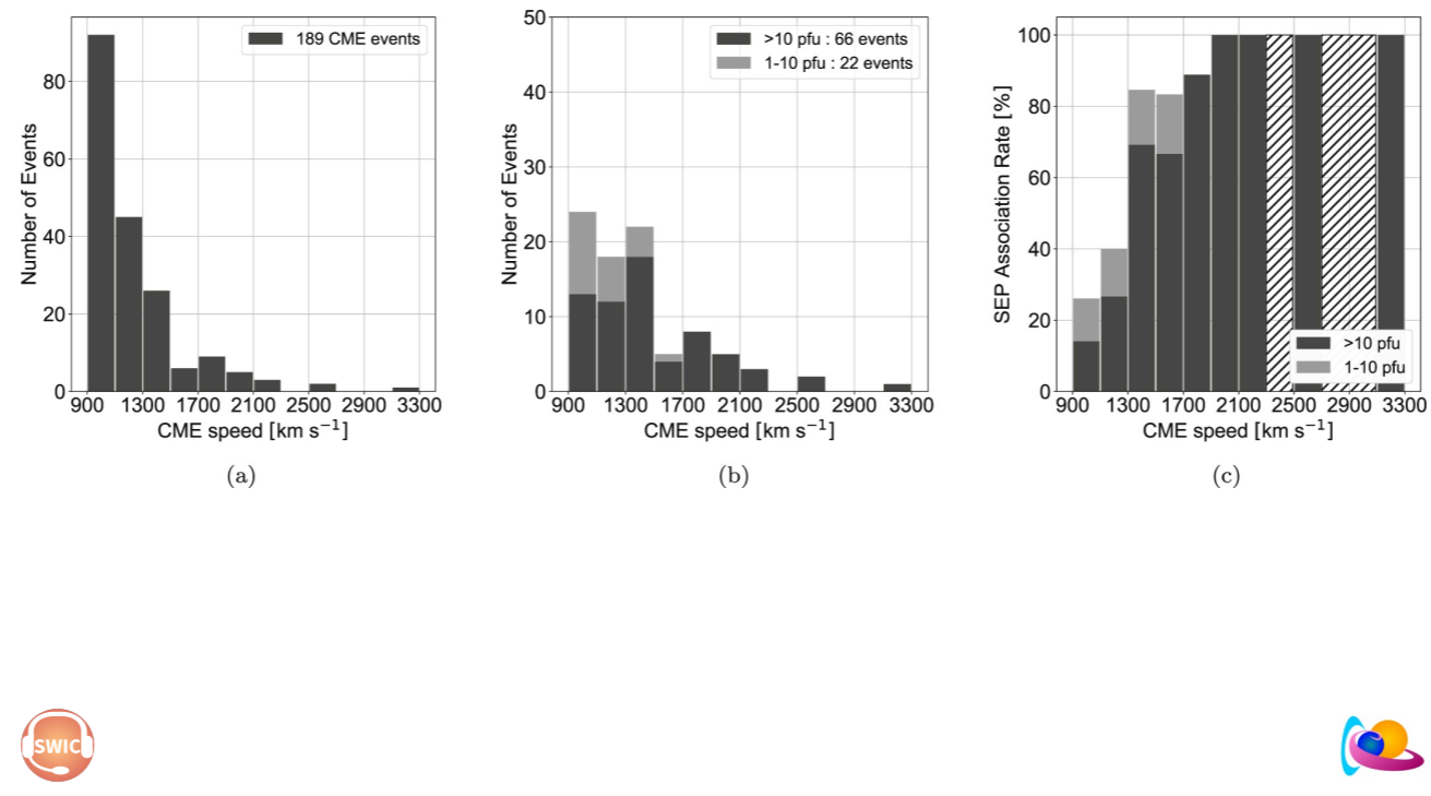
Figure 2. Distribution of CMEs with speed in 200 km s -1 bins. Here we limit the CMEs to those from the source longitudes E20-W100. (a) All the CMEs, irrespective of their associations with SEP events. (b) Only CMEs associated with an SEP event exceeding 10 pfu (black) and between 1 and 10 pfu (gray). (c) The percentage of CMEs associated with an SEP event (the color usage is the same as in (b)). Note that there were no CMEs between 2300 and 2500 km s -1 and between 2700 and 3100 km s -1 , as indicated by the hatched areas in panel (c). As in Figure 1, HiB_N events are excluded ( N \geq 10 in (a), N \geq 10 and N \geq 1 in (b) and (c), for >10 pfu and 1-10 pfu, respectively).
